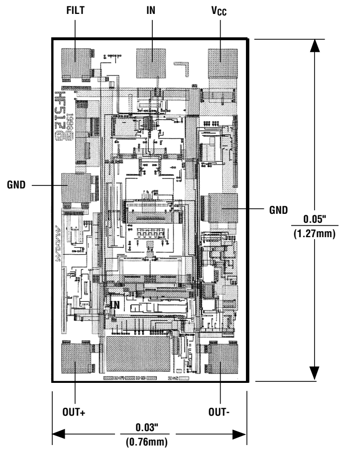
Chip Topography
