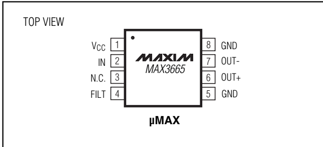
Pin Configuration
